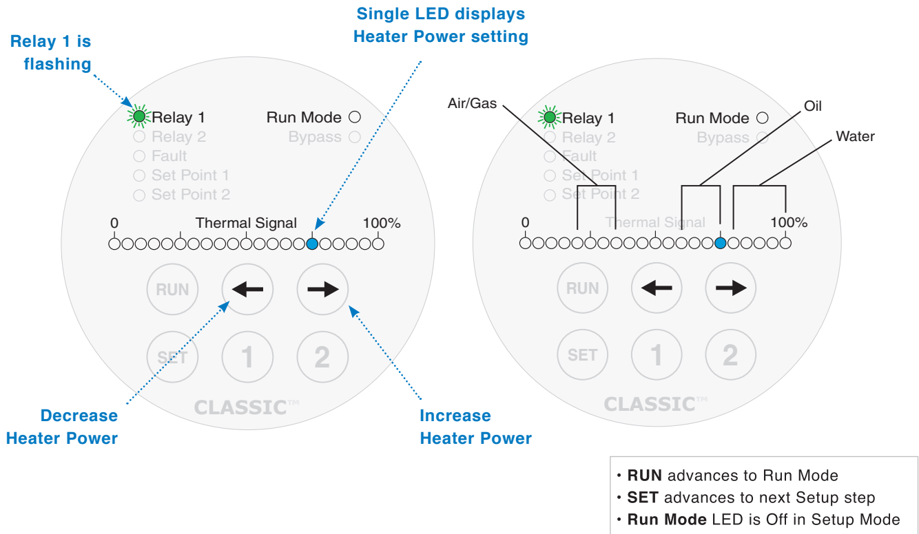
Figure 19 - Setting the Heater Power
