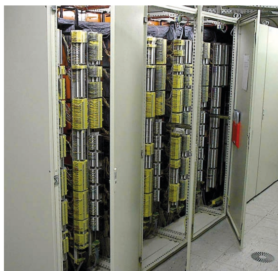
Figure 6 DEHNconnect terminal blocks with integrated surge protection for protecting the complete measuring and control equipment
