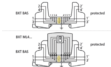
Basic circuit diagram with and without module
