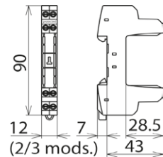
Dimension drawing BXT BAS EX
