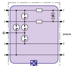
Basic circuit diagram BXT ML2 BD S EX 24
