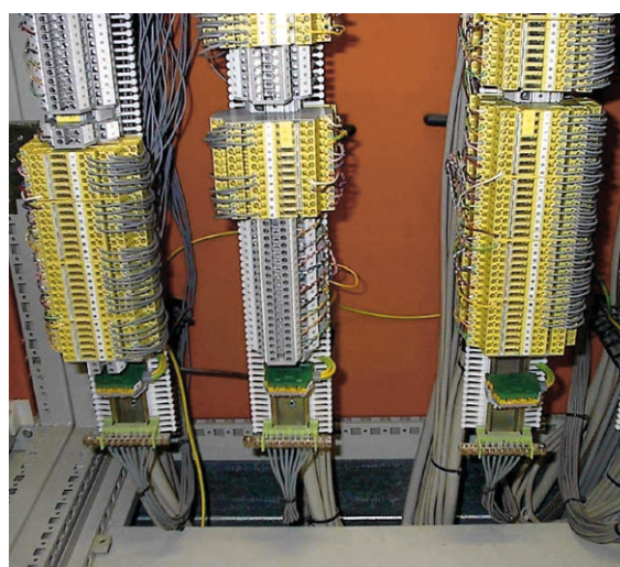
Figure 7 DEHNconnect surge protection devices; lines entering from the double floor
